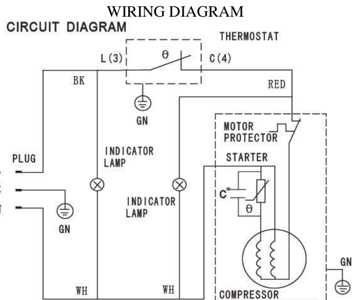
C*: The capacitor is optional according to different compressor model
